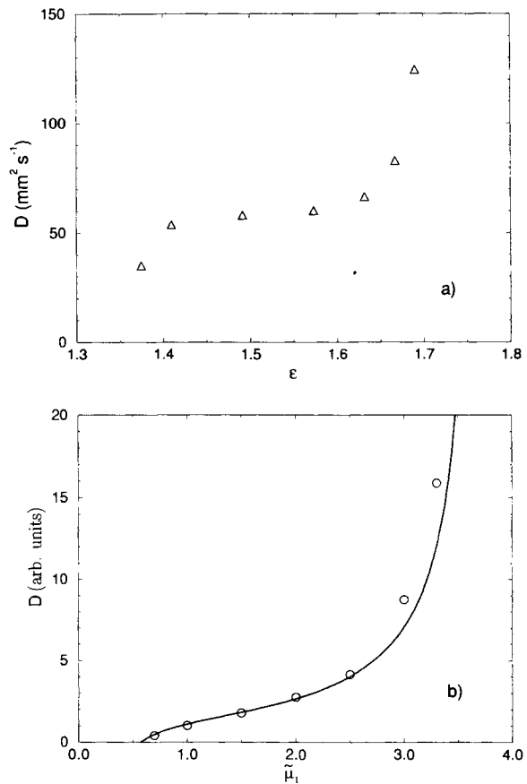
FIG. 4. Evolution of the phase diffusion coefficient D at fixed wave number k . (a) Experimental data ( \Delta ) as a function of \epsilon for k = 1.54 \text{ mm}^{-1} . (b) As a function of \bar{\mu}_1 , calculated analytically (solid line) and numerically ( \circ ). The chosen parameter values are \gamma = 1 , a_1 = 2 , \bar{\mu}_2 = -1 , c_1 = c_2 = 1 , d_1 = d_2 = 0.4 , and k = 2\pi/20 .
