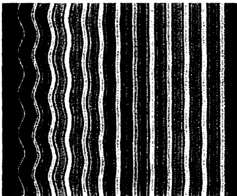
FIG. 3. Spatiotemporal representation of the position of the oil walls when the left boundary is forced to oscillate ( f = 0.01 \text{ Hz} , Z_0 \approx 0.4\lambda , L = 131 \text{ mm} , k = 0.64 \text{ mm}^{-1} , and \epsilon = 0.16 ). 500 s elapse from top to bottom. We found D = 18 \pm 2 \text{ mm}^2/\text{s} , which is of the order of the oil viscosity.
