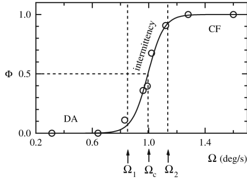
FIG. 4. Mean time fraction \phi of the CF regime as a function of the drum rotation velocity \Omega . Experimental data points (○) and fit by a tanh curve (-).
