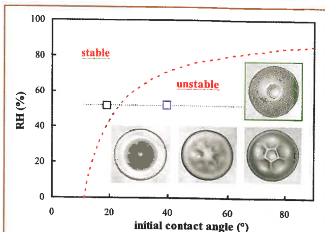
▲ Fig. 1: Diagram showing the instability occurrence for sessile drops during solvent loss under different conditions of initial contact angle ( \theta_0 ) and humidity rate (RH). The red dashed line (theoretical prediction) limits the “stable” and the “unstable” behaviour where drops get strong distortions during the drying process. Insets: images in top view taken at the final stage of the drying process; their location in the diagram corresponds to the conditions ( \theta_0 , RH) necessary to form them. The diameter of the drop contact base is about 5mm.
