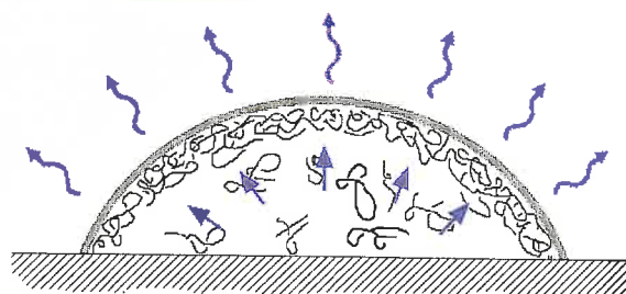
▲ Fig. 2: Schematic illustration of the build up of a glassy “skin” at the drop surface due to the accumulation of the polymer chains near this region.
