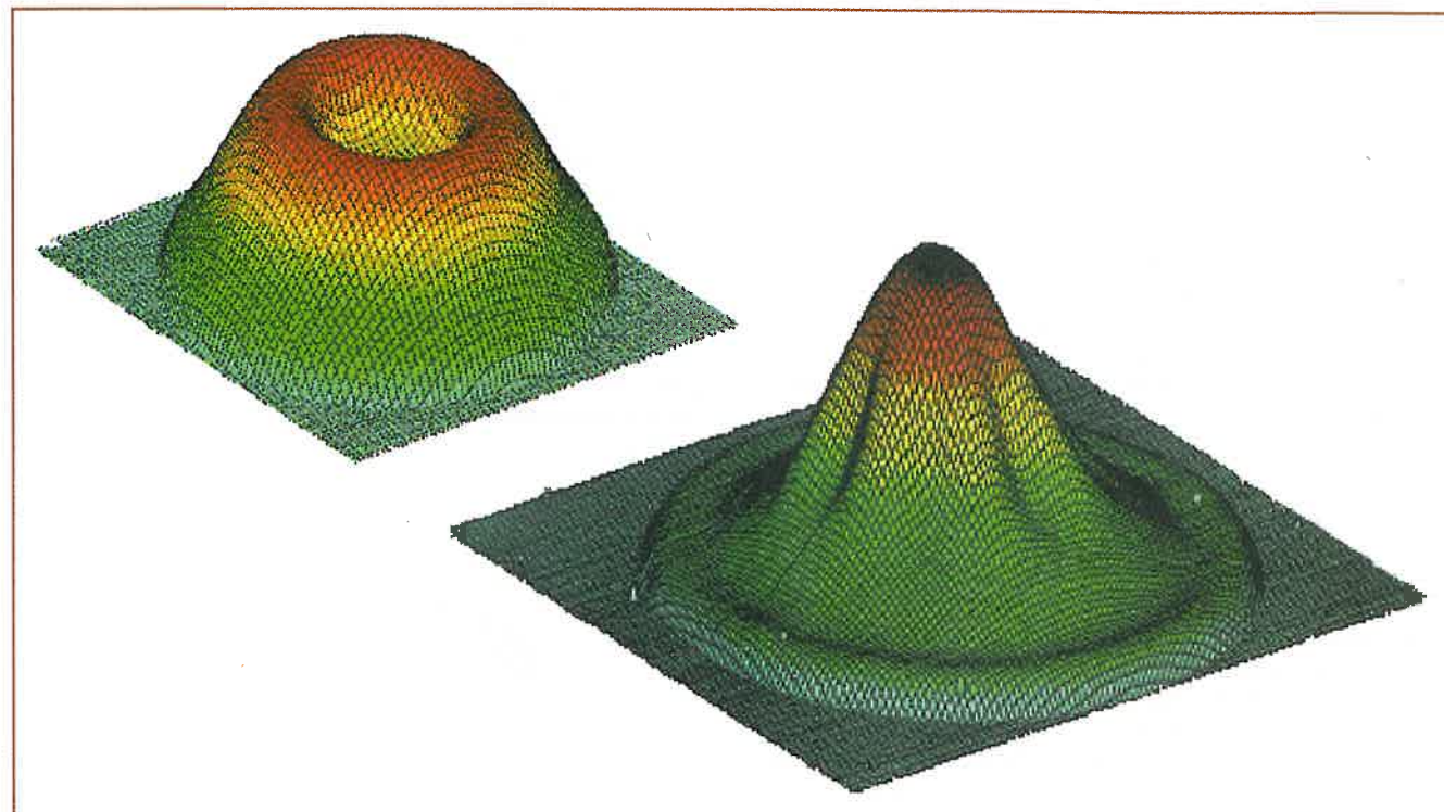
▲ Fig. 4: 3D maps of the drop corresponding to (a) RH=50%; \theta_0=70^\circ ; R_0=2.6\text{mm} and (b) RH=30%; \theta_0=40^\circ ; R_0=2.9\text{mm} . These profiles were measured using a mechanical profilometer (length scales are amplified in the z direction to improve legibility).
