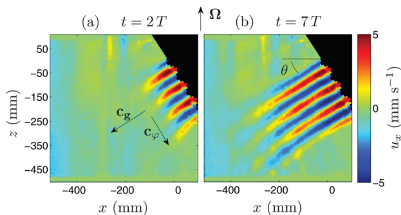
FIG. 2. (Color online) Horizontal velocity field after 2 and 7 periods from the start of the wavemaker for \sigma_0/f = 0.84 . The wavemaker is on the top-right, forcing a wave propagating along \mathbf{c}_g with a phase propagating along \mathbf{c}_\phi .
