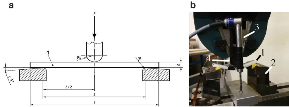
Fig. 4 a According to the ISO 178:2010 standard, the sample dimensions for three-point bending testing were defined as R_1 = 5 \text{ mm} , R_2 = 2.5 \text{ mm} , L = 80 \text{ mm} , h = 4 \text{ mm} , and l = 100 \text{ mm} and b Zwick testing machine: 1—specimen, 2—support, 3—displacement sensor, and 4—punch
