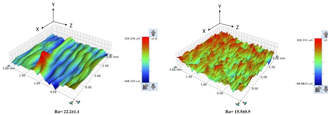
Fig. 9 3D topography profiles of specimen printing by a FFF process and b SLS process. Ra (μm) is the arithmetic mean surface roughness; it is by far the most commonly used parameter in surface finish measurement and for general quality control
