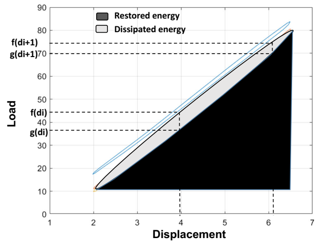
Fig. 15 Illustration of hysteresis cycles (in blue—the first cycle and in gray—the last cycle) and its main parameters in the fatigue test
