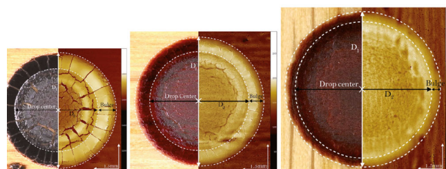
Fig. 16. View of dried blood drip stains with the bulging outer rim, from a healthy volunteer. Droplets of initial diameters of 2.4 mm, and of impact velocities from left to right of 0.74 m/s, 1.87 m/s and 4.75 m/s. On the left side with photography, on the right side with confocal microscopy that gives the 3D features by means of radial cross-sections. Figure reproduced with permission from [65].
