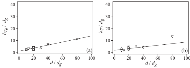
FIG. 13. Dimensionless characteristic length (a) of temperature plateau \delta T_0/d_g and (b) of temperature exponential decrease \lambda_T/d_g as a function of the size ratio d/d_g . (—) Fit of equation (a) \delta T_0 = 1.4d_g + 0.12d and (b) \lambda_T = 2d_g + 0.07d through the data (same symbols as in Figs. 8 and 9).
