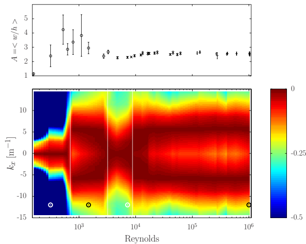
FIG. 4. Top, anisotropy factor A = \langle w/h \rangle computed from experimental power spectra as a function of the Reynolds number (see details in the text and illustration in Fig. 3). Marker shapes ( \circ , \times , + ) represent the different working fluids. Bottom, experimental E_E(k_x) at \theta = 0 as a function of the Reynolds number. Each spectrum is normalized by its maximum. Colors are log scaled. Vertical white lines mark strong transitions in the E_E(k_x) spectrum which highlight parity changes in the structure of the experimental flow. Black and white circles, see Fig. 5.
