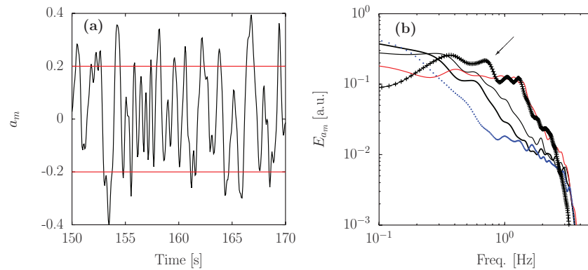
FIG. 8. (a) a_m(t) = \int x dx \int dz \mathbf{v}' \cdot \mathbf{B}^{\mathbf{1mk}_0} with m = 3 and \text{Re} = 10^6 at a fixed angle \varphi (corresponding to the angle of Fig. 2(c)) as a function of time. a_m(t) was computed using \mathbf{v}'(t) from the time-series used in Fig. 5(d) and was finally low-pass filtered at 4 Hz. Horizontal lines, see Fig. 9. (b) Power spectrum E_{a_m}(f) of a_m(t) (+ solid line) for the data shown in (a) and for other Reynolds numbers: \text{Re}/1000 = 41 (thin red/gray line), 21 (thin black line), 12 (thick black line), 7 ( \circ ). The arrow marks the main peak evolution with decreasing Re.
