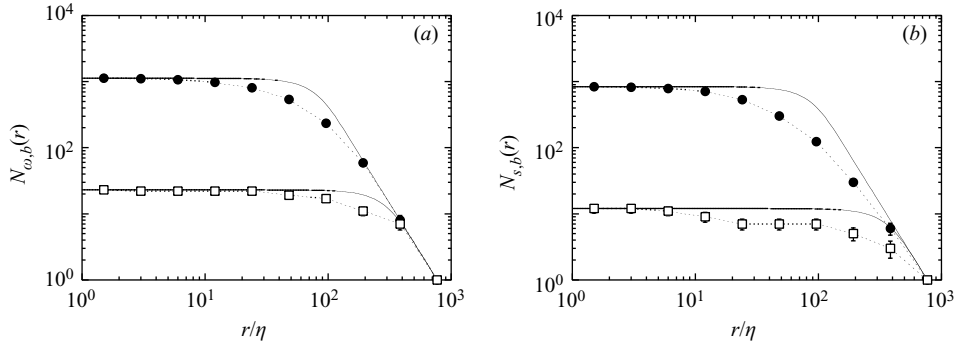
FIGURE 15. Box counts of the set of baricentres of the intense structures. (a) Vorticity structures. \bullet , |\omega| \geq 6\omega' ; \square , |\omega| \geq 12\omega' . (b) Strain structures. \bullet , |s| \geq 4.2s' ; \square , |s| \geq 8.5s' . The solid lines are the corresponding Poisson box countings N_0 , from (3.4).
