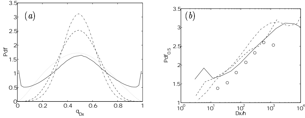
Figure 2.- (a) Pdfs of the breakdown coefficients of the surrogate averaged dissipation, for several averaging lengths. Re_\lambda = 1600 . —, \Delta x/\eta = 3 ; ·····, 24; ----, 380; -·-·-, 3000. (b) Midpoint value of the pdf as a function of averaging length. Lines are as in table 1; \circ , Van Atta and Yeh (1975). Re_\lambda = 2600 .
