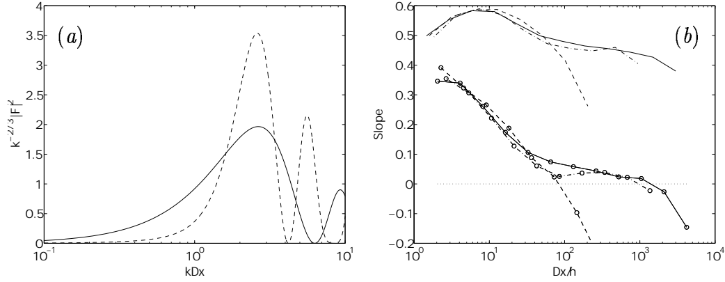
Figure 13.- (a) Filtered inertial spectra kE(k)|F(k)|^2 , with E = k^{-5/3} . —, for the difference operator (4.5); ----, for the ‘sharp’ filter (5.7). (b) Slope of the conditional mean values. Simple lines are the same as in figure 11(a). Those with symbols are computed with (5.7).
