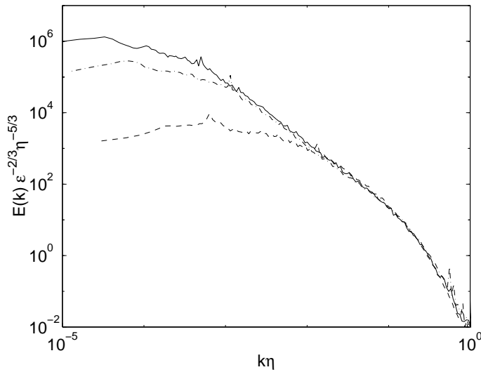
Figure 1.- One-dimensional power spectra of the three data sets analyzed in this paper. Line types as in table 1.
