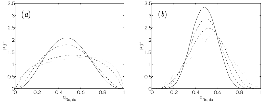
Figure 4.- Conditional pdfs of the dissipation breakdown coefficients, for several dissipations and length scales. Re_\lambda = 1600 . (a) \Delta x/\eta = 23 , corresponding to an abscissa of 0.5 in figure 3. Dissipations correspond to the following ordinates in figure 3: — , -0.94 ; - - - , -0.82 ; - - - - , -0.59 ; ····· , -0.36 . (b) \Delta x/\eta = 1500 (abscissa, 1.2). Ordinates: — , -0.36 ; - - - , -0.24 ; - - - - , -0.12 ; ····· , 0.
