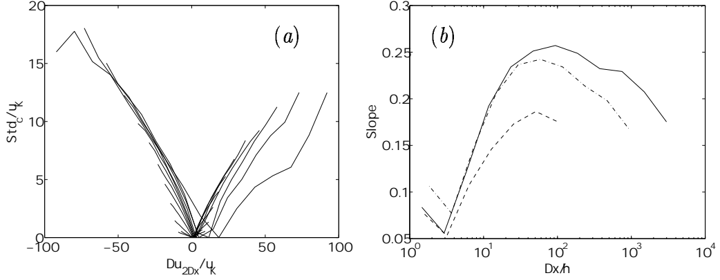
Figure 12.- (a) ‘Coherent’ conditional standard deviation of the velocity increments, as a function of the conditioning velocity increments. Data as in figure 10. Each line represents a different \Delta x . Re_\lambda = 1600 . (b) Slope of the coherent standard deviation in (a) with respect to the conditioning velocity increments. Lines as in table 1. The slopes of the positive and negative branches of (a) have been averaged for this figure.
