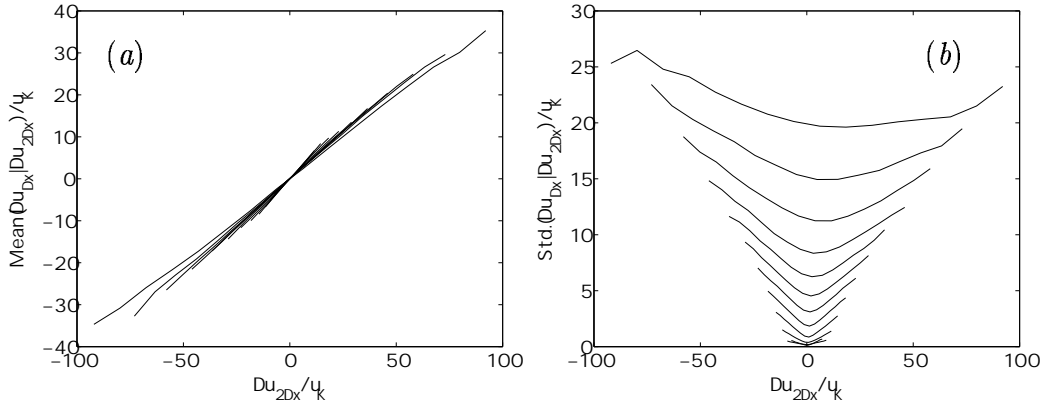
Figure 10.- (a) Mean value of \Delta u_{\Delta x} , conditioned on the velocity increment \Delta u_{2\Delta x} of its parent interval. (b) Standard deviations. In both figures \Delta x/\eta ranges from 1.5 to 3000, increasing by factors of 2 in the direction of longer lines. Re_\lambda = 1600 .
