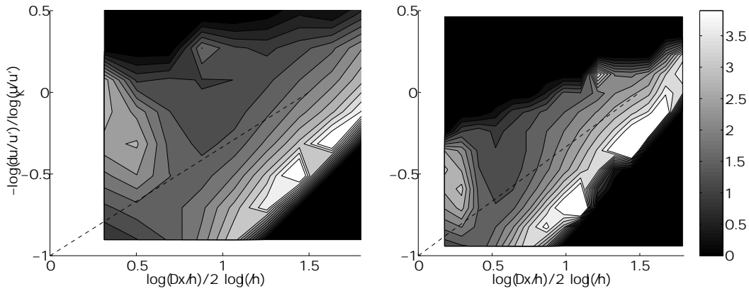
Figure 3.- Midpoint value of the conditional pdfs of the breakdown coefficients for the surrogate averaged dissipation, as a function of the averaging length and of the surrogate velocity increment. (a) Re_\lambda = 155 . (b) Re_\lambda = 1600 .
