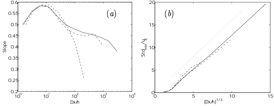
Figure 11.- (a) Slope of the conditional mean values in figure 10(a), d\langle\Delta u_{\Delta x}|\Delta u_{2\Delta x}\rangle/d\Delta u_{2\Delta x} . (b) Minimum conditional standard deviations in figure 10(b). Lines as in table 1. The slope of the dotted line is 1.6.
