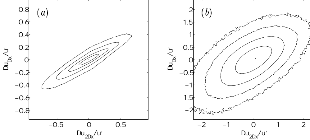
Figure 7.- Joint pdfs of the velocity increments across centred segments whose lengths differ by a factor of two. Re_\lambda = 1600 . (a) \Delta x/\eta = 6 . (b) \Delta x/\eta = 90 . Contour lines are logarithmically spaced by factors of 10.
