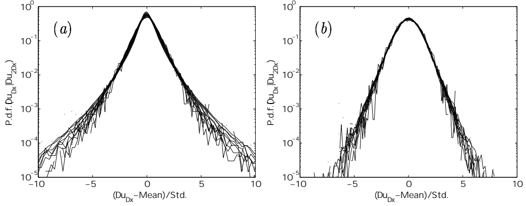
Figure 9.- Normalized pdfs of \Delta u_{\Delta x} conditioned on the velocity increment \Delta u_{2\Delta x} of its parent interval. Re_\lambda = 1600 . (a) \Delta x/\eta = 12 , |\Delta u_{2\Delta x}/u_K| = 1 - 14 . (b) \Delta x/\eta = 750 , |\Delta u_{2\Delta x}/u_K| = 4 - 60 .
