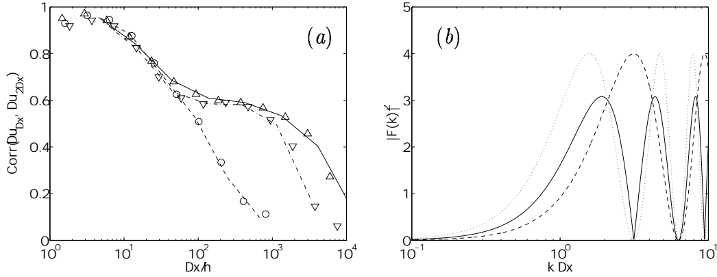
Figure 8.- (a) Correlation coefficients for the joint pdfs in figure 4, as a function of the separation distance. Lines are as in table 1. (b) Transfer functions for the difference operator. ---- , |F(k\Delta x)|^2 ; ..... , |F(2k\Delta x)|^2 ; ——— , |F(k\Delta x)F^*(2k\Delta x)| .
