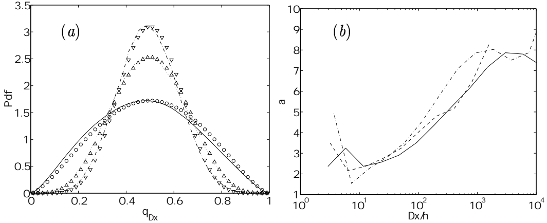
Figure 5.- (a) Approximation of the experimental pdfs of the dissipation breakdown coefficients by symmetric Beta distributions having the same maxima. Re_\lambda = 1600 . —, \Delta x/\eta = 23 ; ·····, 370; - - -, 6000. (b) Best value of \alpha for the Beta approximation of the breakdown pdfs. Lines as in table 1.
