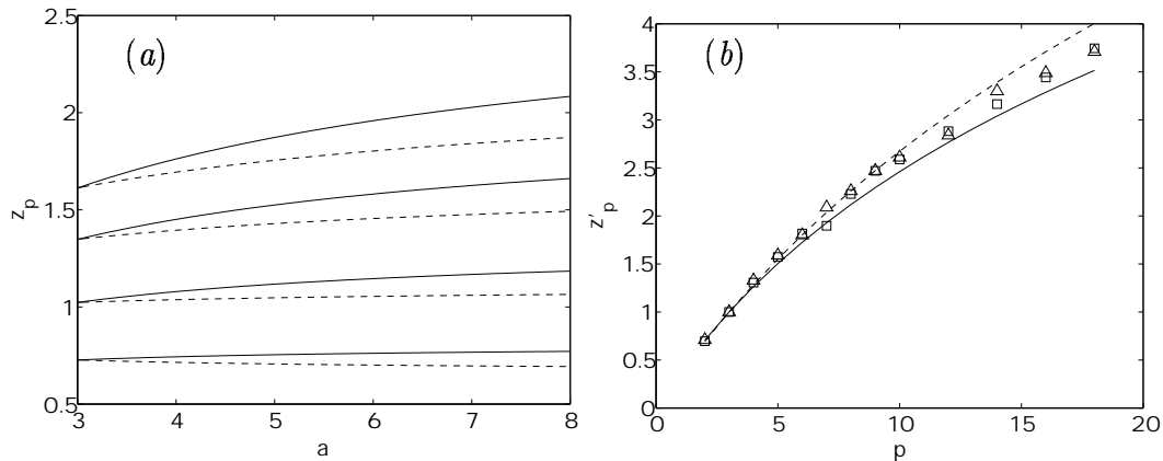
Figure 6.- (a) Scaling exponents for the Beta distributions, as a function of the parameter \alpha . p = 2, 4, 6, 8 , in increasing order. — , true exponent; ---- , extended self-similarity. (b) Scaling exponents of the longitudinal velocity structure functions. \square , Herweijer and van de Water (1994); \triangle , Anselmet et al. (1984). Re_\lambda \approx 500 - 800 in both cases; — , Beta distribution with \alpha = 5 ; ---- , \alpha = 8 .
