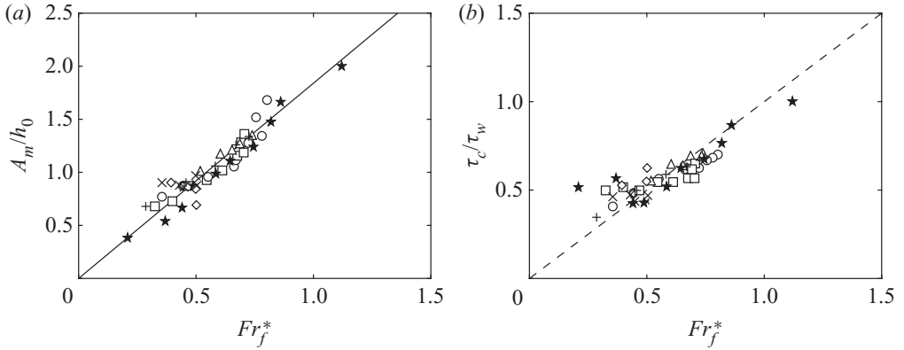
FIGURE 14. (a) Normalized maximum amplitude A_m/h_0 as a function of the modified local Froude number Fr_f^* = v_{f,m}/\sqrt{g(h_0 + A_m)} based on the velocity of solitary waves, for all the experiments listed in table 1 (symbols) together with the best linear fit A_m/h_0 = 1.84 Fr_f^* (—). (b) Time ratio \tau_c/\tau_w as a function of Fr_f^* . The dashed line corresponds to \tau_c/\tau_w = Fr_f^* .
